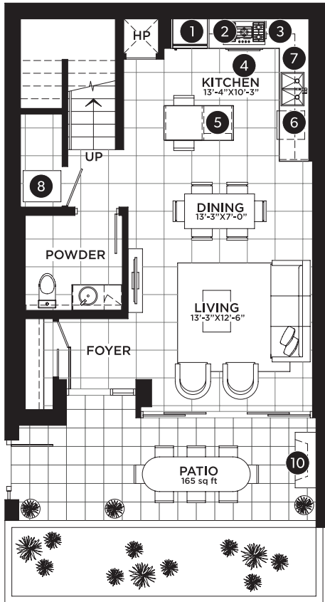
GROUND FLOOR 570 sq ft
