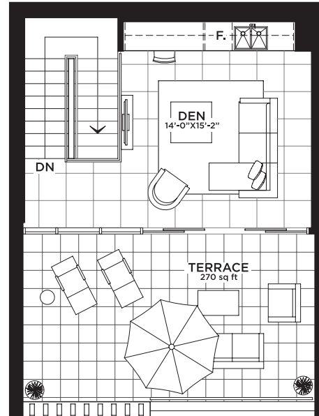
UPPER FLOOR 275 sq ft
